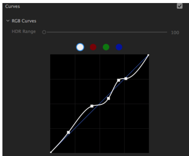
RGB curves
